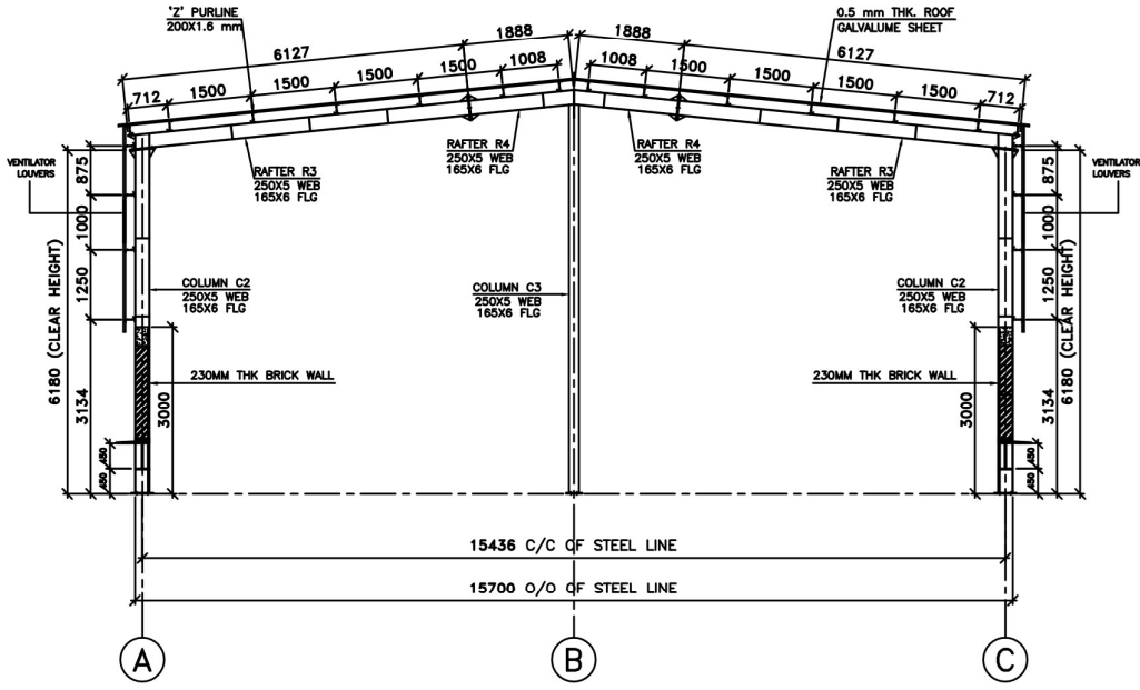
PORTAL FRAME AT GRID 1 & 4.
