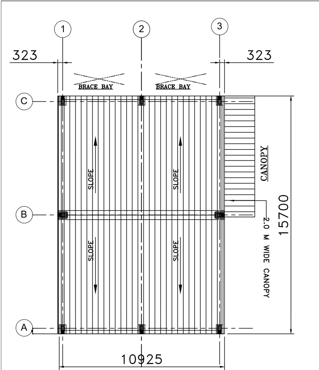
ROOF LAYOUT PLAN
