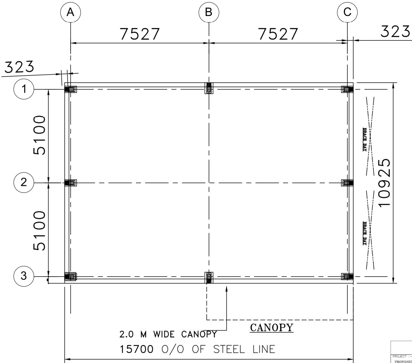
LAYOUT PLAN
